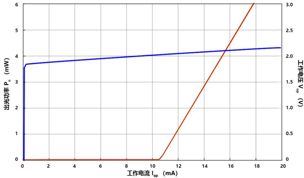
HGLD-650TO5.6-JP-5mW PIV 测试曲线
